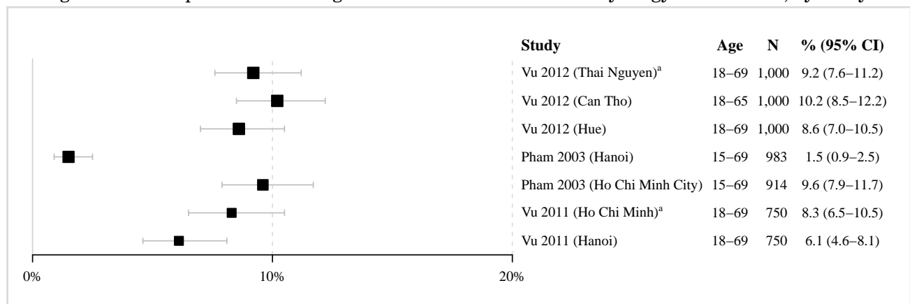
Figure 24: HPV prevalence among women with normal cervical cytology in Viet Nam, by study
