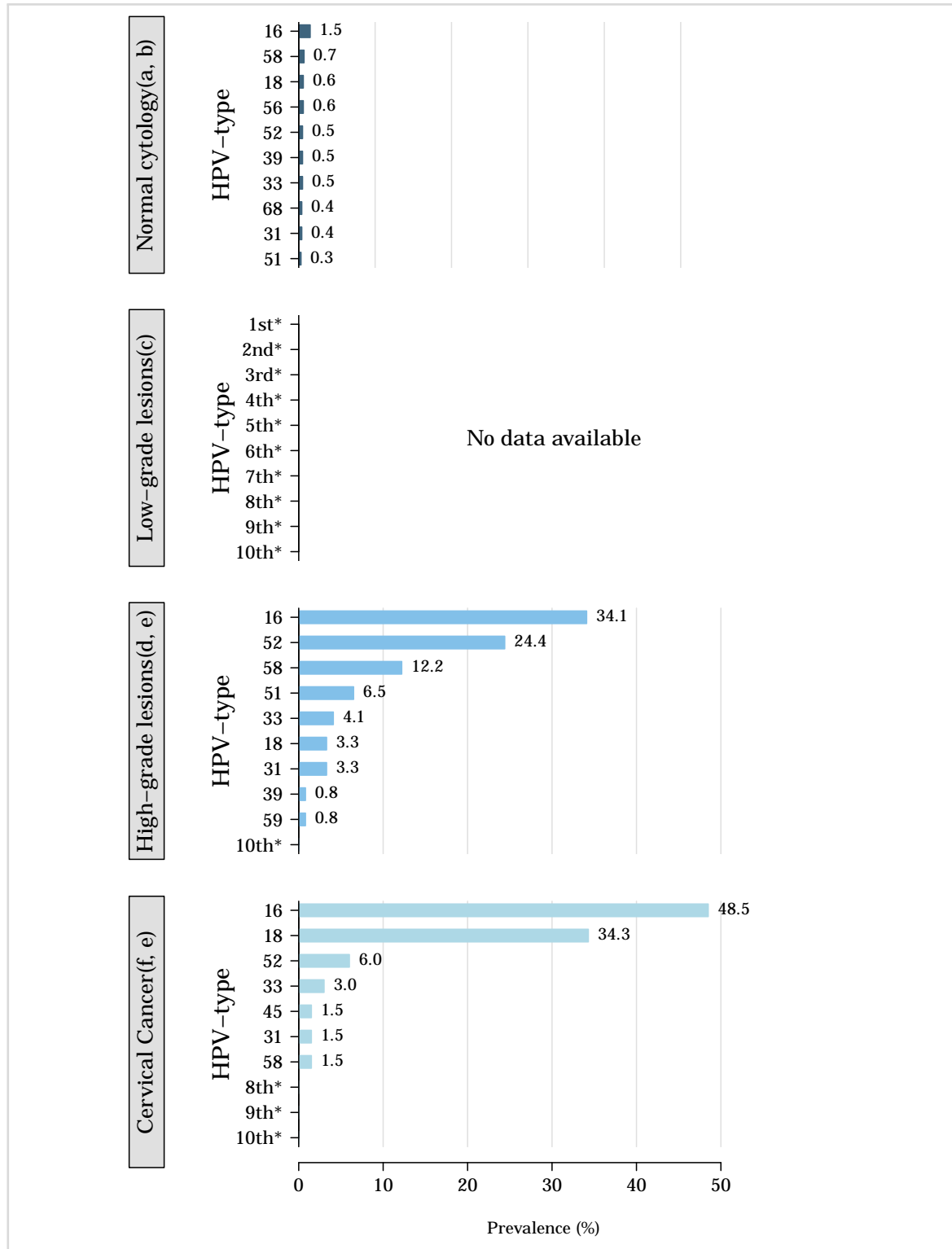
Figure 29: Comparison of the ten most frequent HPV oncogenic types in Viet Nam among women with and without cervical lesions
