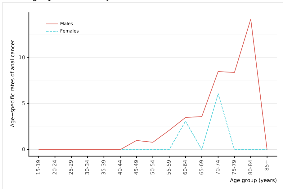
Figure 17: Age-specific mortality rates of anal cancer in Oman (estimates for 2020)
