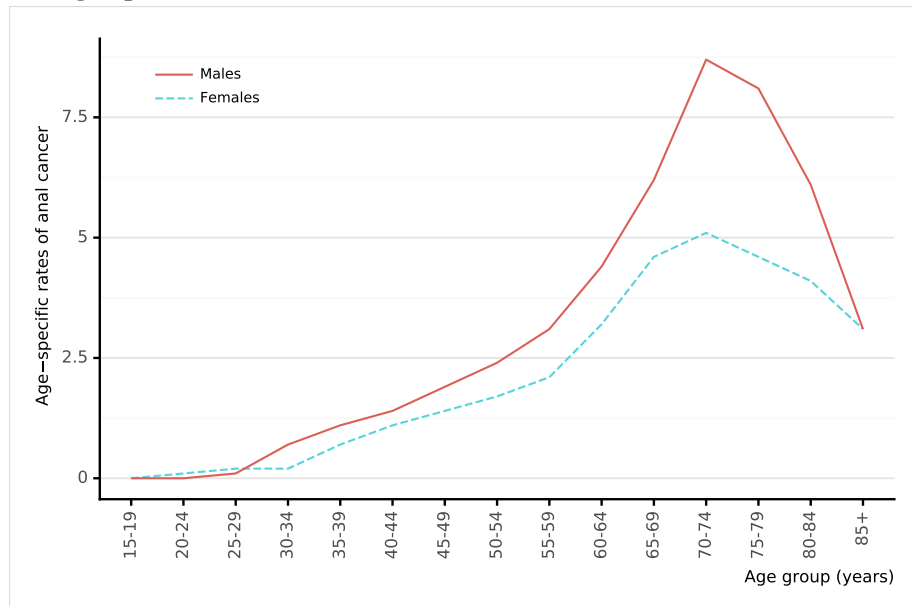
Figure 15: Age-specific incidence rates of anal cancer in Uzbekistan (estimates for 2020)
